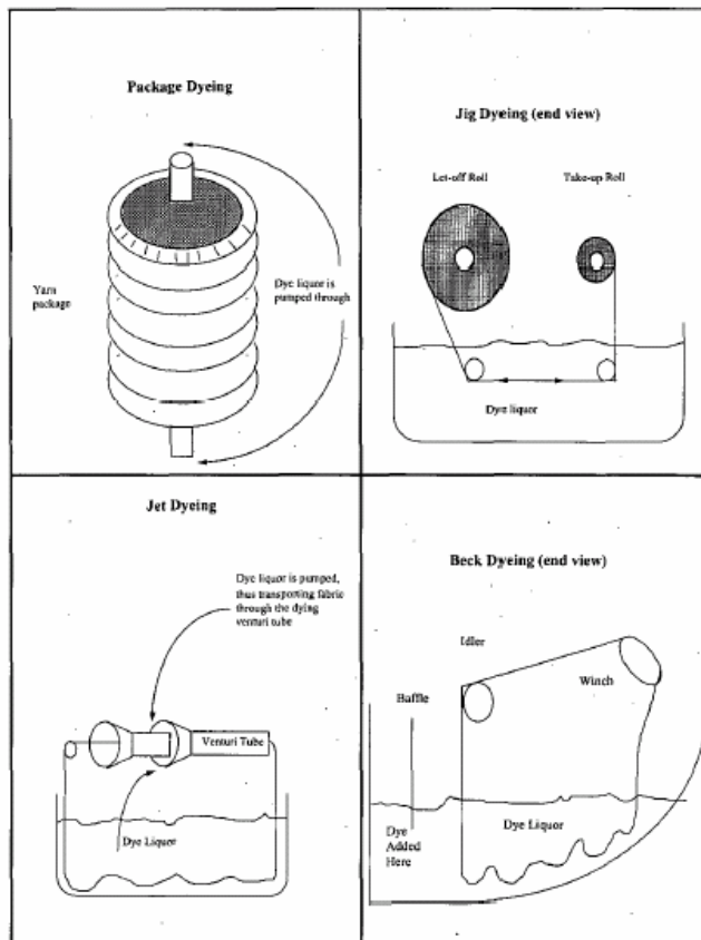
Figure 1. Common Textile Dyeing Methods. Source: EPA, 1997.
